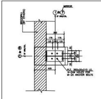
DETAIL D3 (AS DRAWN) (2 Nos. REQD.) (A-01) DETAIL D3X (OPP. HAND) (2 Nos. REQD.) (A-01)
