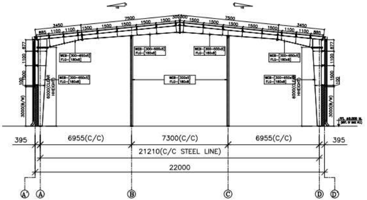
END-WALL FRAME PLAN (FOR GRID LINE 1 & 7)
