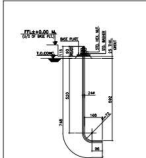
M-24 ANCHOR BOLT DETAIL (56 Nos. REQD.)
