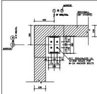
DETAIL D1 (AS DRAWN) (2 Nos. REQD.) (A-01) DETAIL D1X (OPP. HAND) (2 Nos. REQD.) (A-01)
