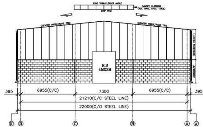
END WALL SHEETING ELEVATION (FOR GRID LINE 7)
