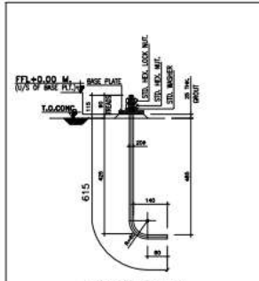
M-20 ANCHOR BOLT DETAIL (16 Nos. REQD.)
