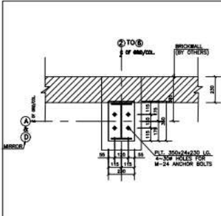
DETAIL D2 (AS DRAWN) (2 Nos. REQD.) (A-01) DETAIL D2X (OPP. HAND) (2 Nos. REQD.) (A-01)
